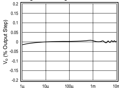
Long Term Settling Time
