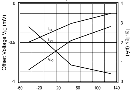
I_{BI} , I_{BN} , V_{IO} vs. Temperature
