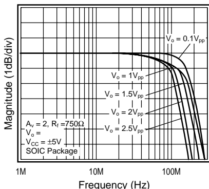
Figure 7: Frequency Response vs. V_o
