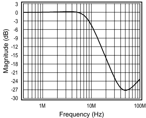
Figure 16: Lowpass Response
