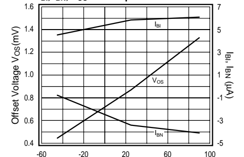
I_{BI} , I_{BN} , V_{OS} vs. Temperature
