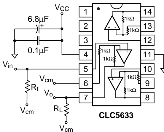
FIGURE 3. DC Coupled, A_v = +2V/V Configuration
