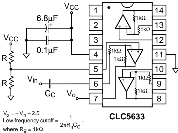
FIGURE 4. AC Coupled, A_v = -1/V Configuration
