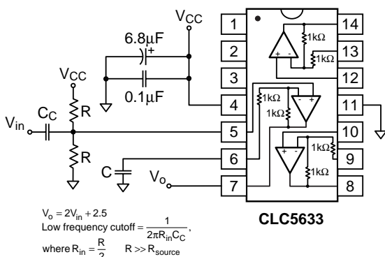
FIGURE 6. AC Coupled, A_v = +2/V Configuration
