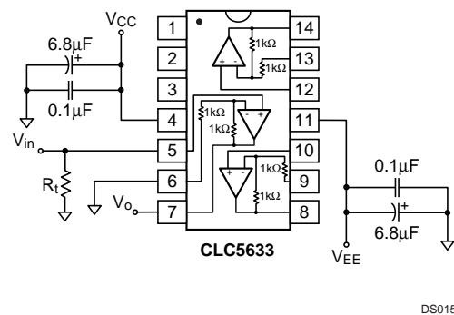
FIGURE 9. Dual Supply, A_v = +2/V Configuration
