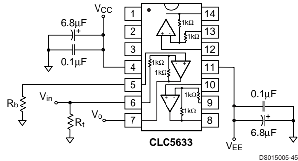
FIGURE 7. Dual Supply, A_v = -1/V Configuration
