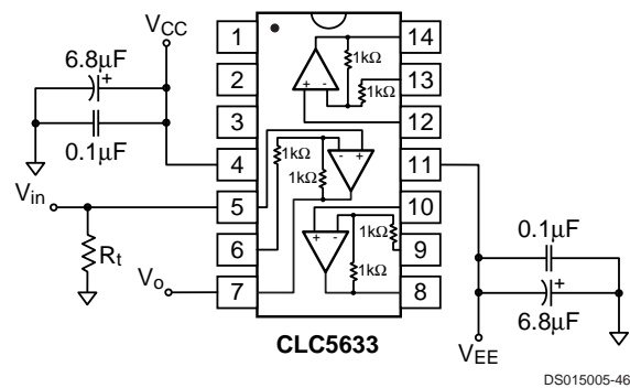
FIGURE 8. Dual Supply, A_v = +1/V Configuration
