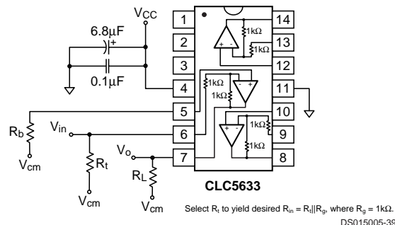
FIGURE 1. DC Coupled, A_v = -1V/V Configuration
