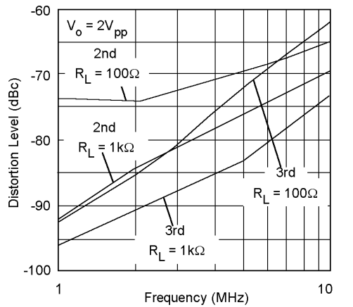
2nd & 3rd Harmonic Distortion vs. Frequency
