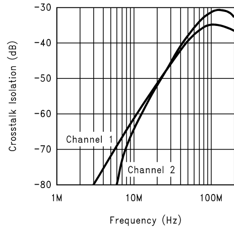
Channel-to-Channel Crosstalk
