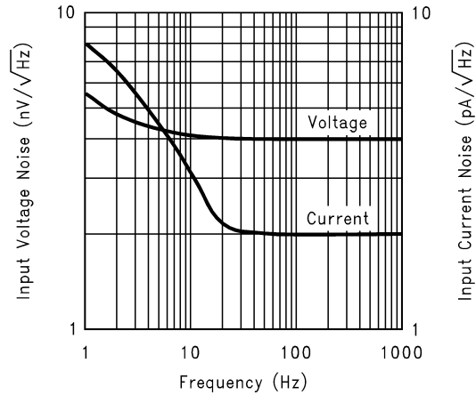
Equivalent Input Noise
