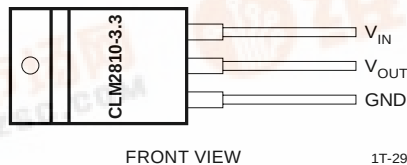
PLASTIC PACKAGE TO-220
