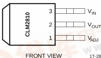
PLASTIC DD PACKAGE
