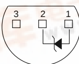
TO-92 (N-SUFFIX) BOTTOM VIEW
