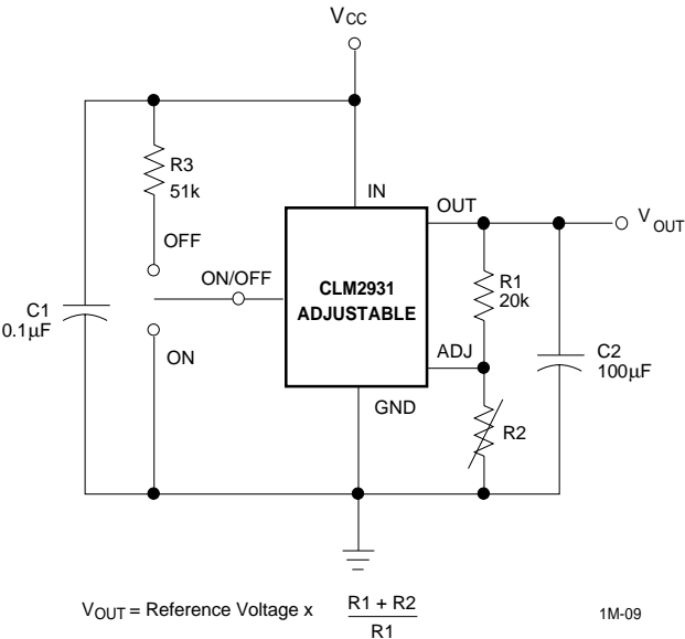
CLM2931 ADJUSTABLE OUTPUT
