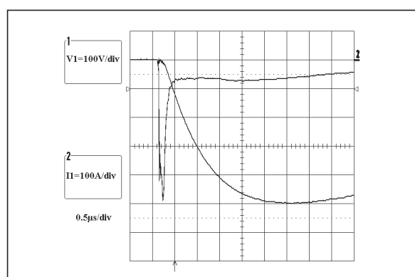
Fig. 12 : CLP270M response to a negative surge.
