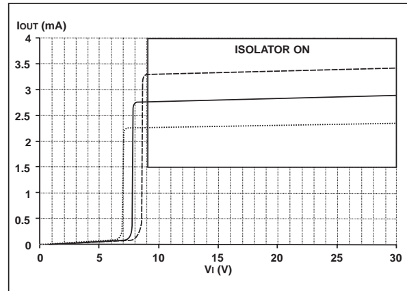
Fig. 5: Transconductance characteristic
