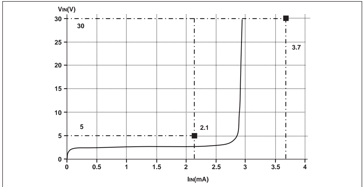
Fig. 1: Typical input characteristics of each CLT3-4 channel
