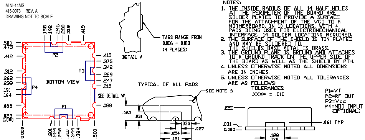
PHYSICAL DIMENSIONS
