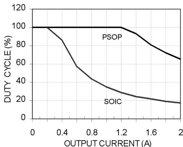
Figure 13. Duty Cycle vs. Output Current (Temp=70°C)
