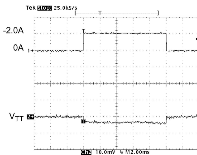
Figure 11. Line Transient (0A to 2.0A Source)
