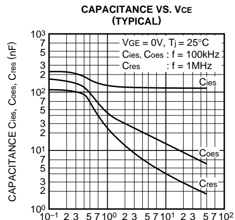
COLLECTOR-EMITTER VOLTAGE V_{CE} (V)
