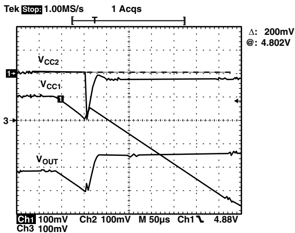
Figure 5. V_{CC1} falling from 0V to 5V ( V_{CC2} = 5V ). Ch1 and Ch2: V_{CC1} and V_{CC2} , offset = 5V. Ch3: V_{OUT} , offset = 5V.
