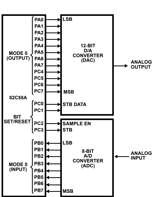
FIGURE 21. DIGITAL TO ANALOG, ANALOG TO DIGITAL
