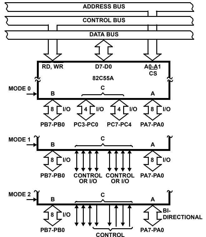
FIGURE 3. BASIC MODE DEFINITIONS AND BUS INTERFACE
