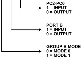
FIGURE 11. MODE CONTROL WORD
