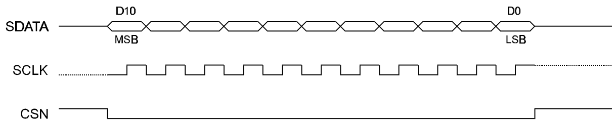
Figure 10: Serial Port Timing Diagram
