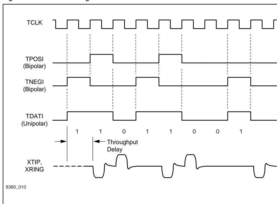
Figure 2-5. Transmitter Signals
