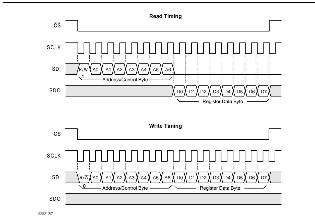
Figure 4-6. Host Serial Port Timing Diagram
