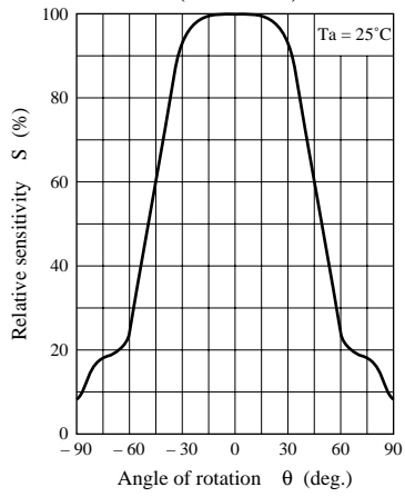
Directivity characteristics (Receiver)
