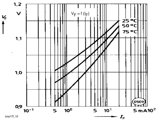
Figure 10. Forward Voltage
