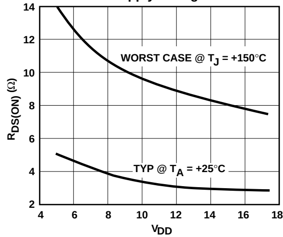
Output Resistance (Output Low) vs. Supply Voltage
