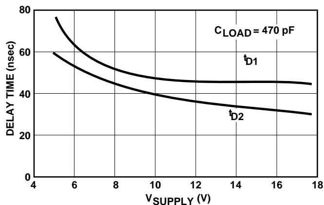
Propagation Delay Time vs. Supply Voltage
