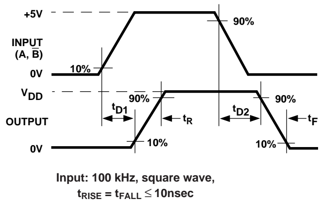
Figure 1. Switching Time Test Circuit
