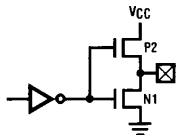
a. Standard Push-Pull Output
