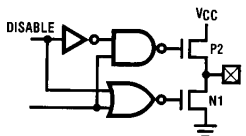
d. Standard TRI-STATE "L" Output
