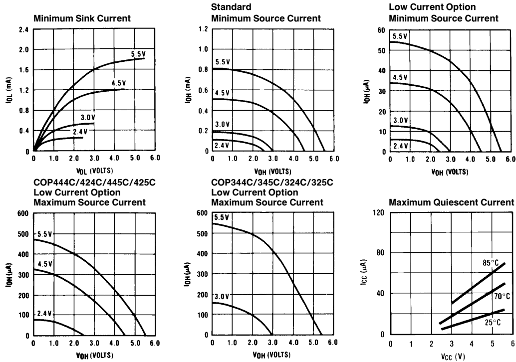
FIGURE 12. Input/Output Characteristics
