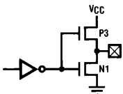
b. Low Current Push-Pull Output
