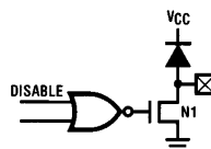
f. Open Drain TRI-STATE "L" Output
