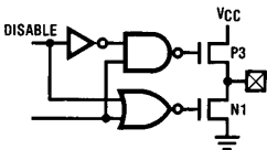
e. Low Current TRI-STATE "L" Output
