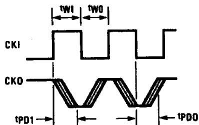
FIGURE 3b. CKO Output Timing
