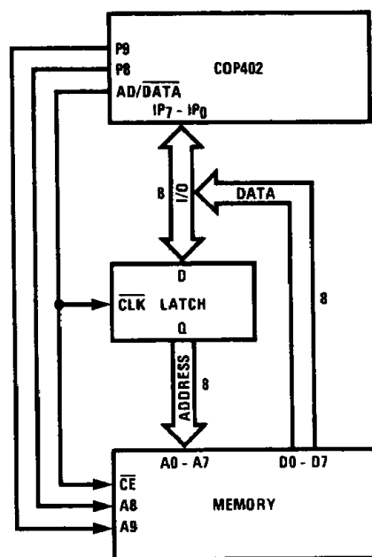
FIGURE 9. External Memory Interface to COP402
