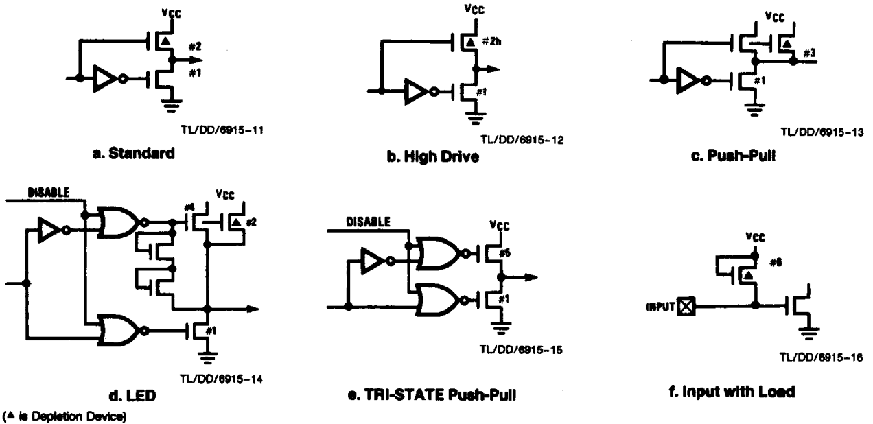
FIGURE 10. Input/Output Configurations
