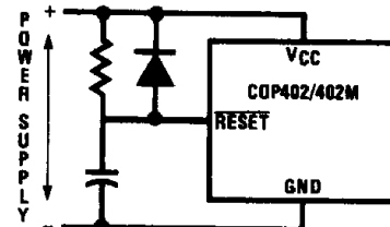
RC \geq 5 \times \text{Power Supply Rise Time} TL/DD/6915-8 FIGURE 7. Power-Up Clear Circuit
