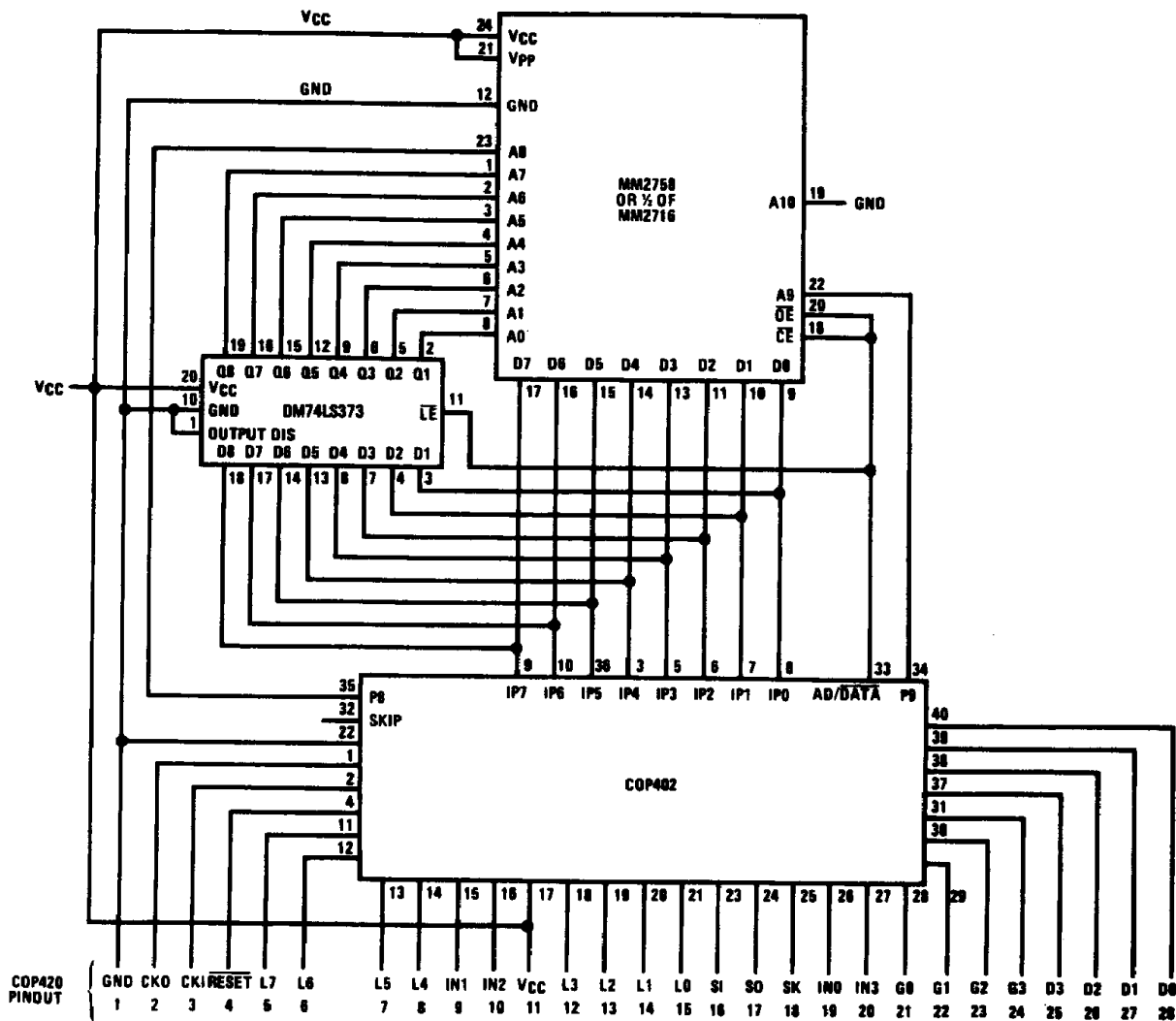
FIGURE 13. COP402 Used to Emulate a COP420
