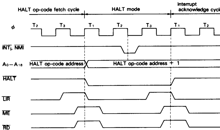
Figure 18 HALT Timing
