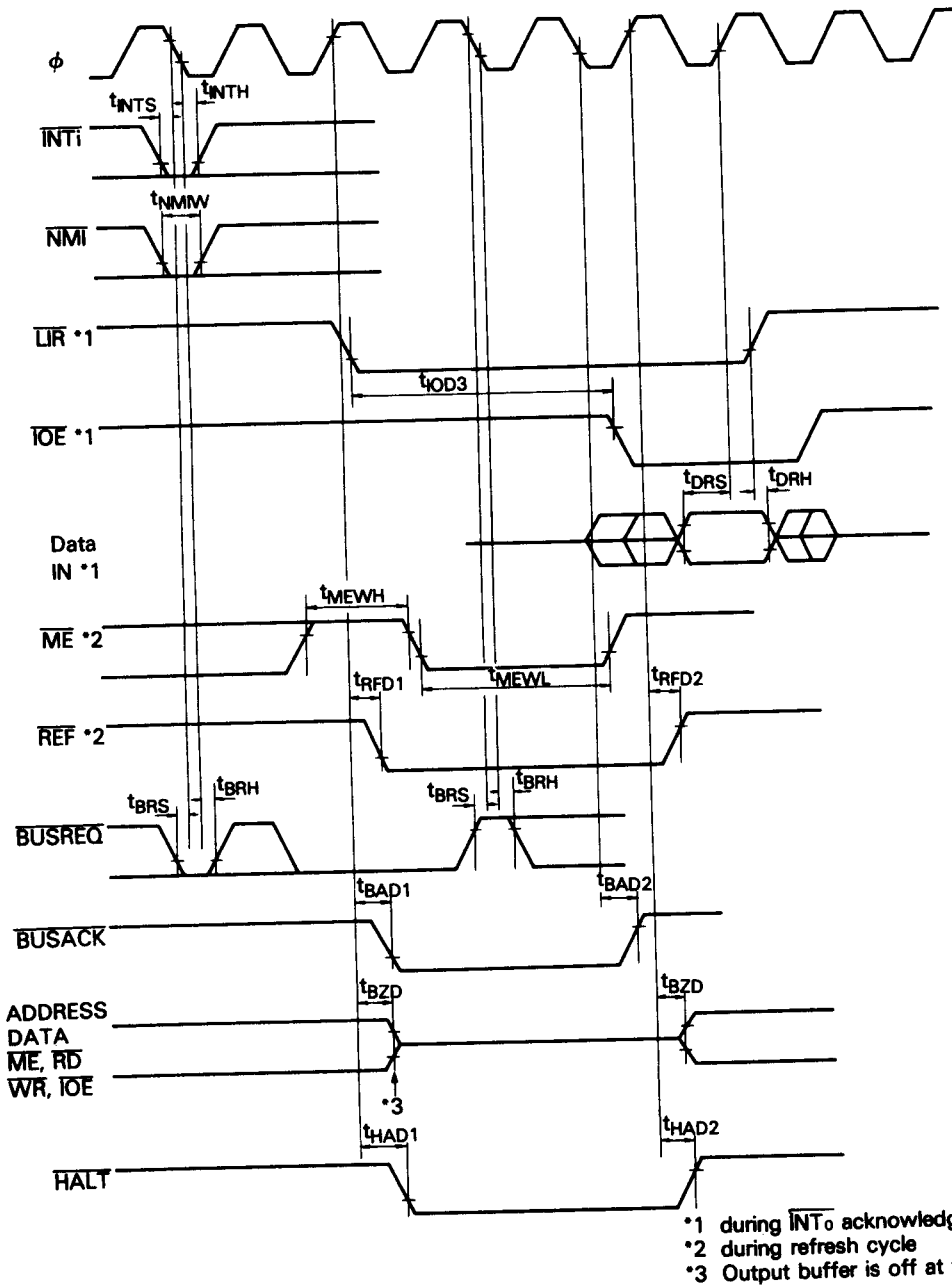
Figure 1 CPU Timing (2)
