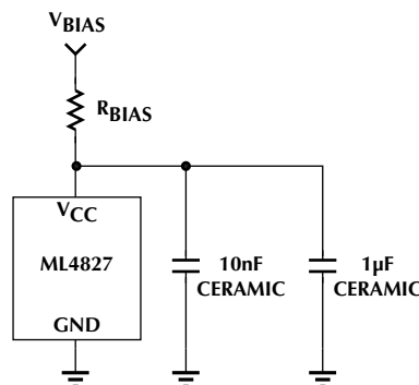
Figure 4. External Component Connections to V_{\text{CC}}
