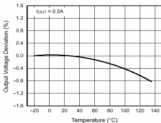
Fig. 7 – Temperature Stability
