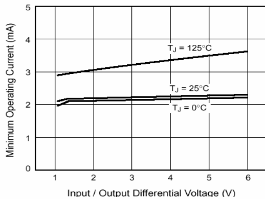
Fig. 1 – Minimum Load Current (Adjustable Version)
