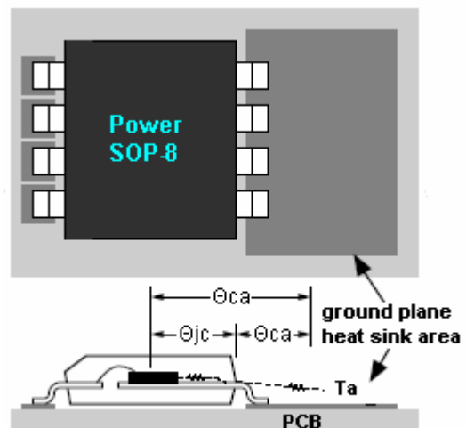
Thermal Resistance
