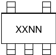
5-Lead SC-70 (MCP9701)
