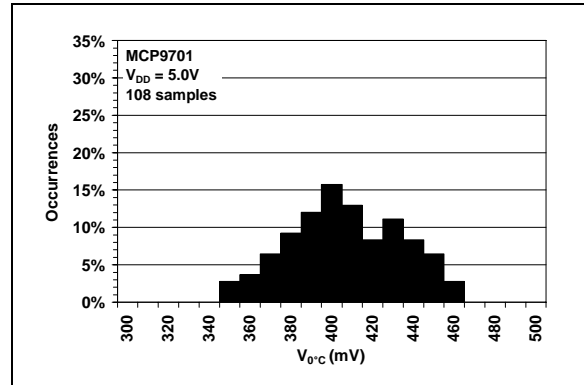
FIGURE 2-10: Occurrences vs. Temperature Coefficient (MCP9701).
