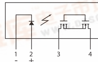
CPC1926Y Pinout
