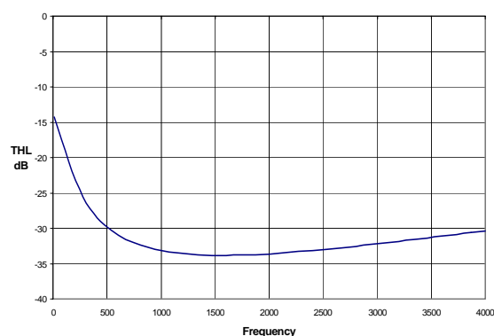
Figure 12. Trans-Hybrid Loss
