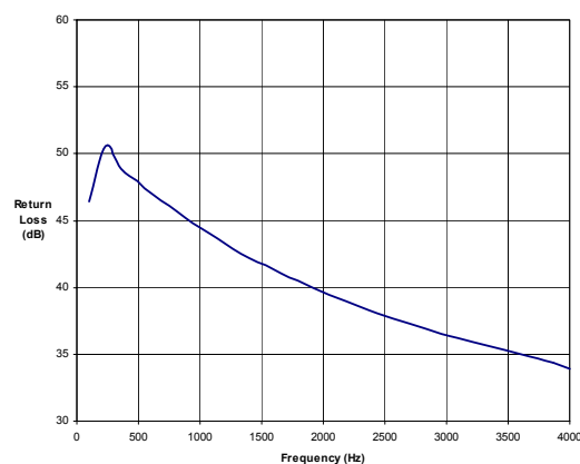
Figure 13. Return Loss
