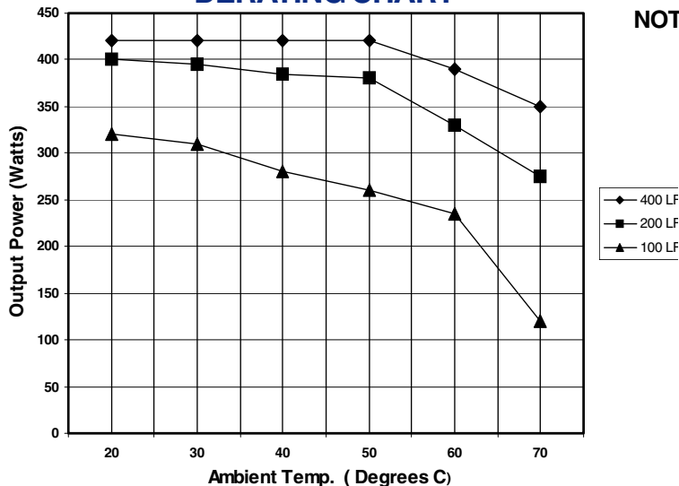
DERATING CHART
