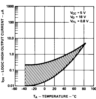
Figure 4. Typical Logic High Output Current vs. Temperature.
