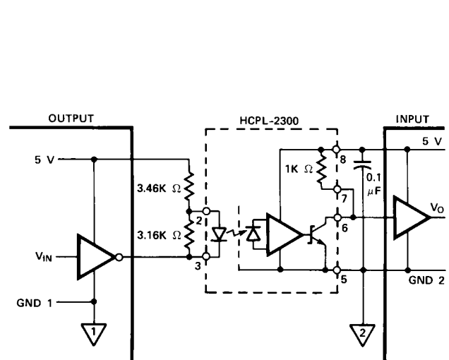
Figure 14. Series Drive from Open Collector TTL/LSTTL
