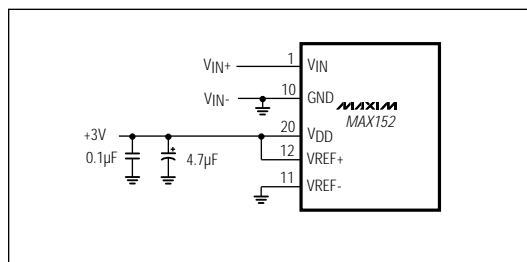
Figure 7a. Power Supply as Reference
