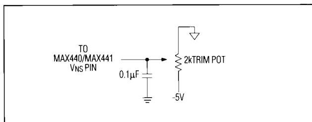
Figure 5. VNS Pin-Voltage Adjustment
