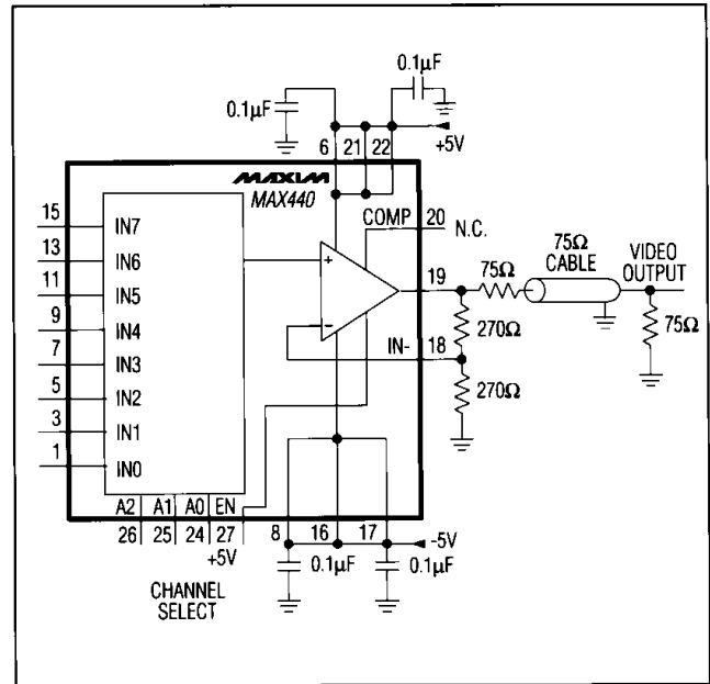
Figure 3. Coaxial-Cable Driver
