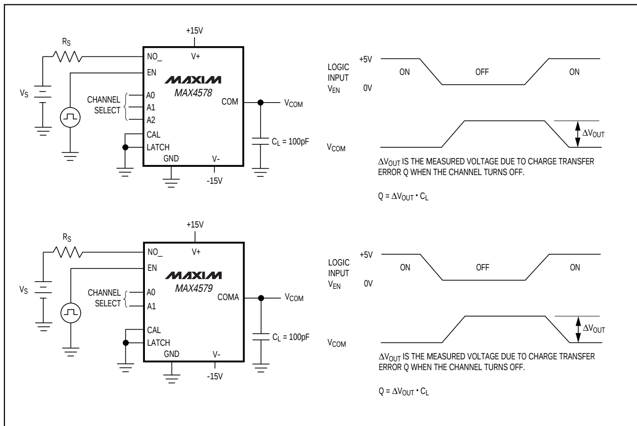
Figure 4. Charge Injection
