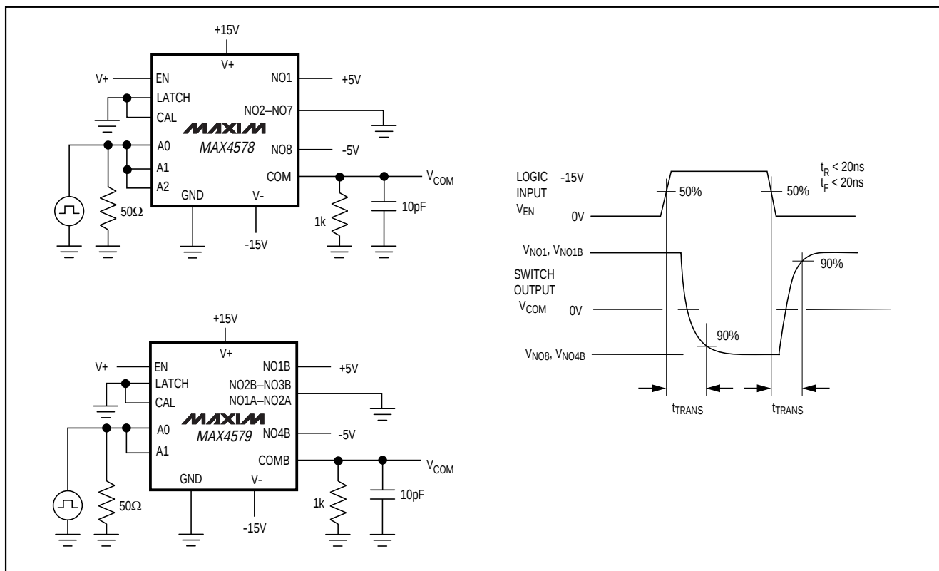
Figure 1. Transition Time
