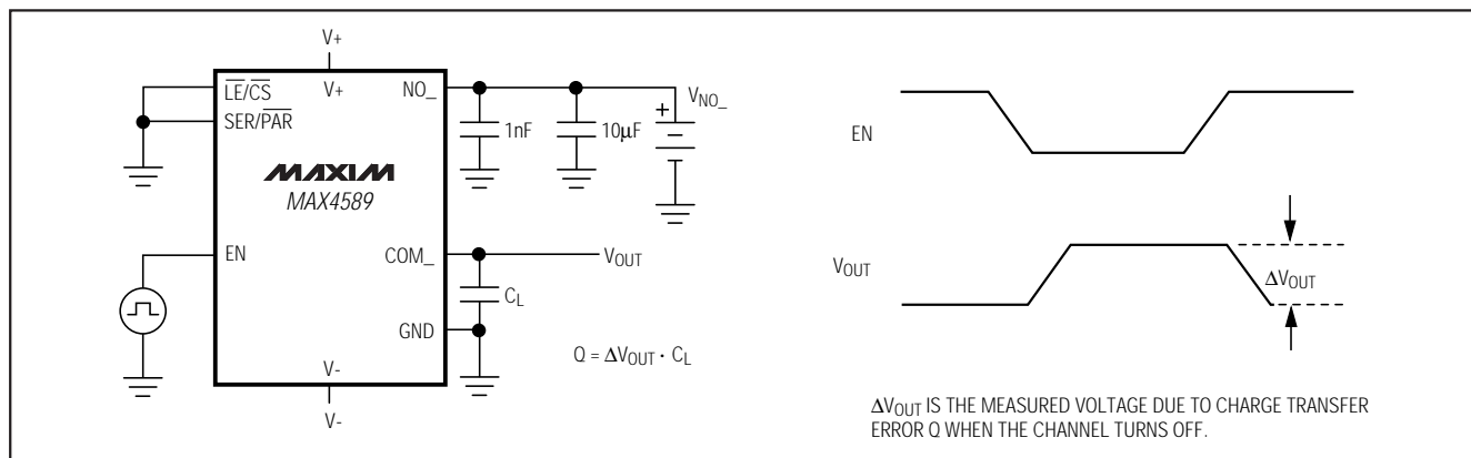
Figure 3. Charge Injection
