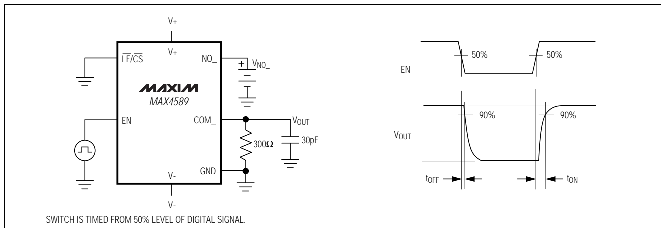
Figure 1. Turn-On/Turn-Off Time
