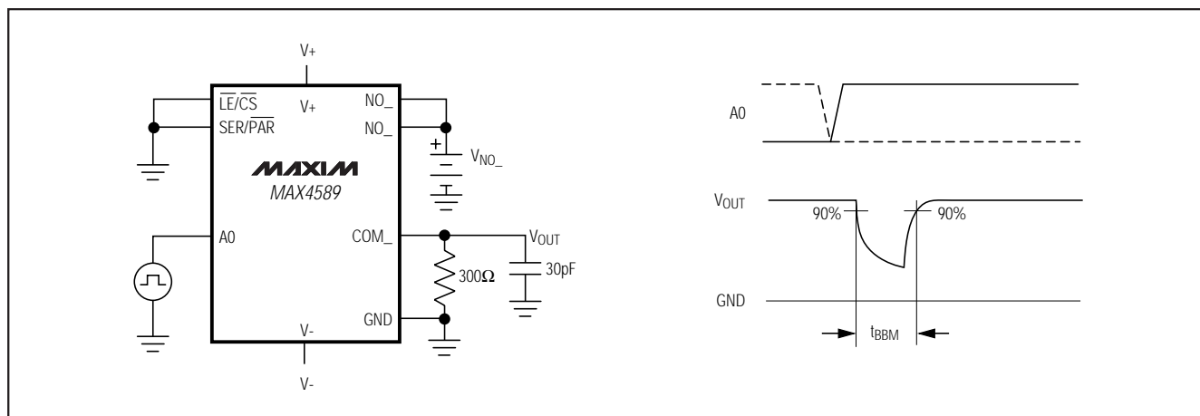
Figure 2. Break-Before-Make Time Delay
