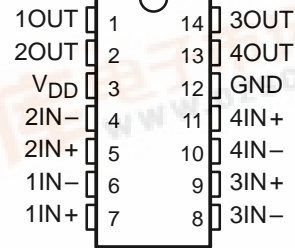
PW PACKAGE (TOP VIEW)
