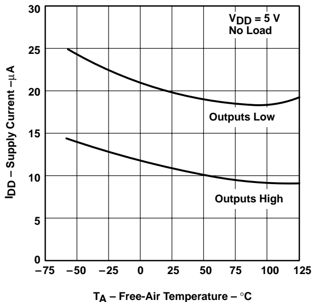
T_A – Free-Air Temperature – ^\circ\text{C} Figure 24
