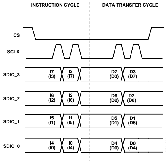
Figure 44. 4-Bit Serial Mode Write Timing—Clock Stall Low
