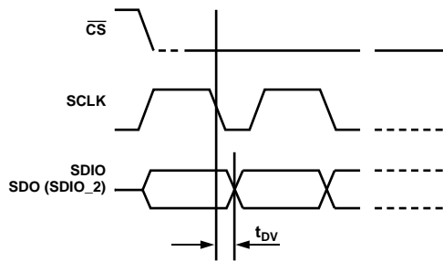
Figure 41. Timing Diagram for Data Read for Serial I/O Port
