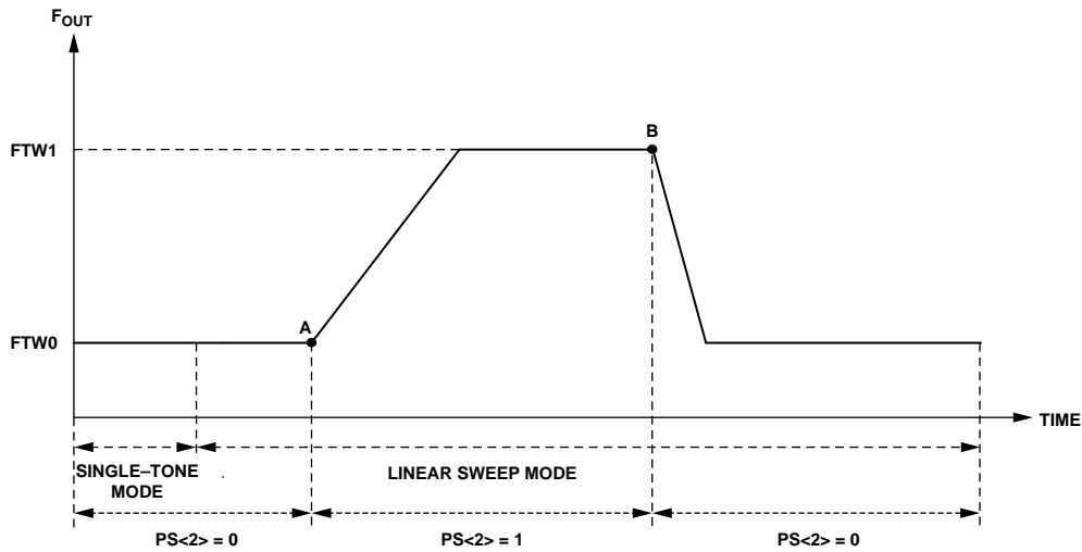
AT POINT A: LOAD RISING RAMP RATE REGISTER, APPLY RISING DFTW. AT POINT B: LOAD FALLING RAMP RATE REGISTER, APPLY FALLING DFTW.
