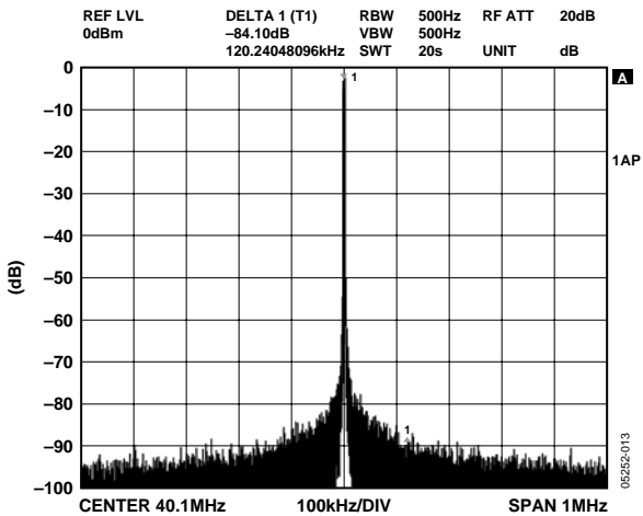
Figure 13. f_{OUT} = 40.1 MHz, f_{CLK} = 500 MSPS, NBSFDR, \pm 1 MHz
