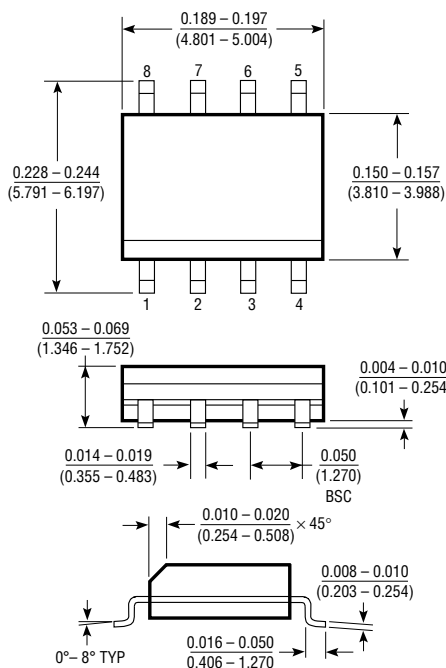
S8 Package, 8-Lead Plastic SOIC
