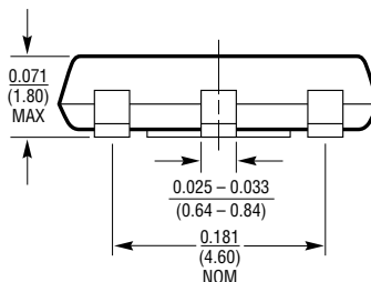
ST Package, 3-Lead SOT-223
