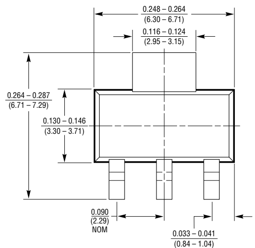
ST Package, 3-Lead SOT-223
