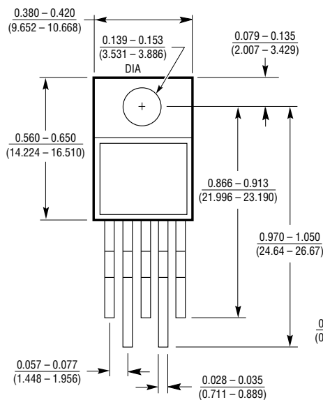
T Package, 5-Lead TO-220
