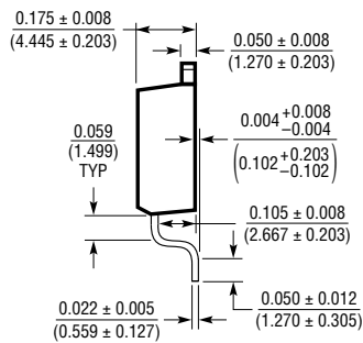
Q Package, 5-Lead DD
