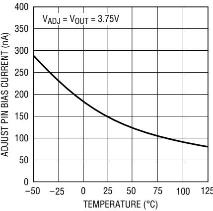
Adjust Pin Bias Current
