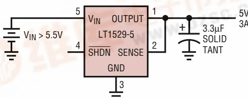
5V Supply with Shutdown
