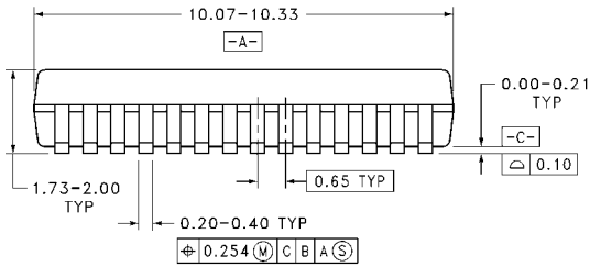
28-Lead Shrink Small Outline Package (SSOP), EIAJ TYPE II, 5.3mm Wide Package Number MSA28
