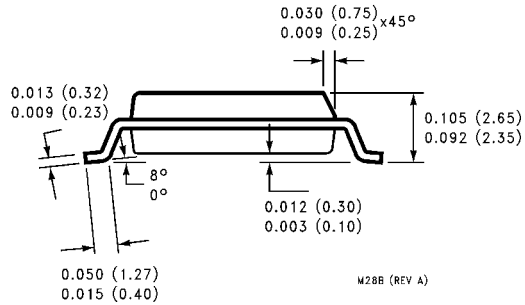
28-Lead Small Outline Integrated Circuit (SOIC), MS-013, 0.300" Wide Body Package Number M28B
