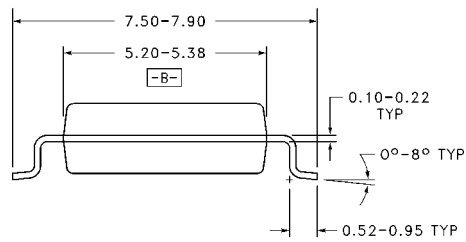
28-Lead Shrink Small Outline Package (SSOP), EIAJ TYPE II, 5.3mm Wide Package Number MSA28
