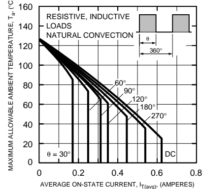
MAXIMUM ALLOWABLE AMBIENT TEMPERATURE (RECTANGULAR WAVEFORM)
