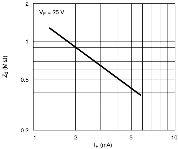
Dynamic Impedance vs. Regulator Current
