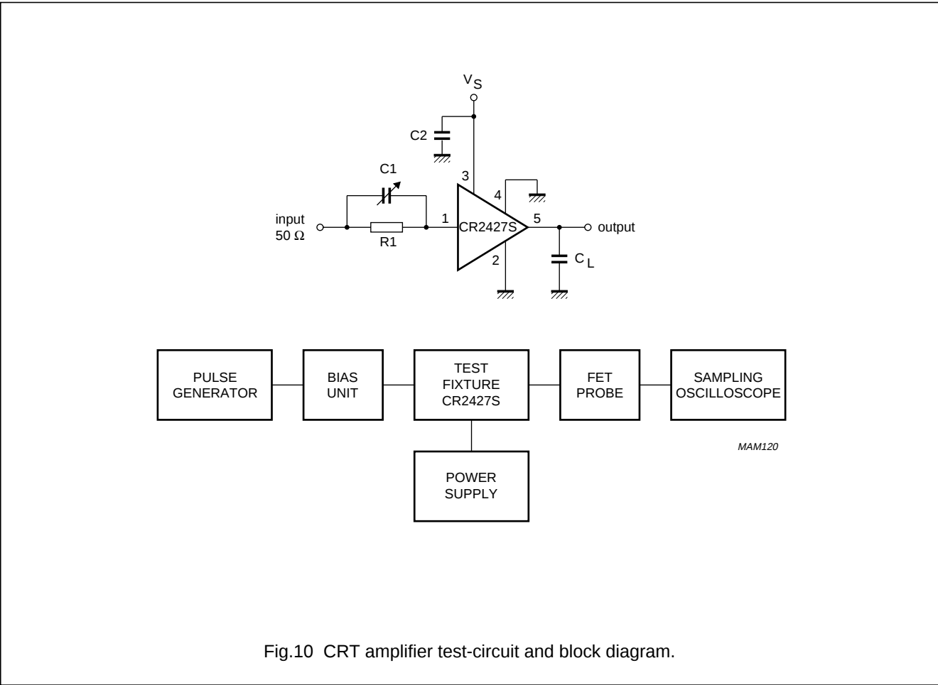
Components used in test-circuit (see Fig.10)
