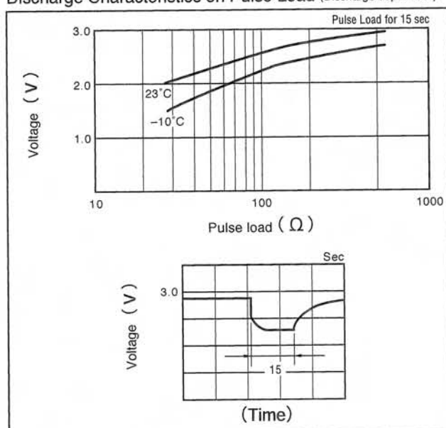
Discharge Characteristics on Pulse Load (Discharge depth 40%)
