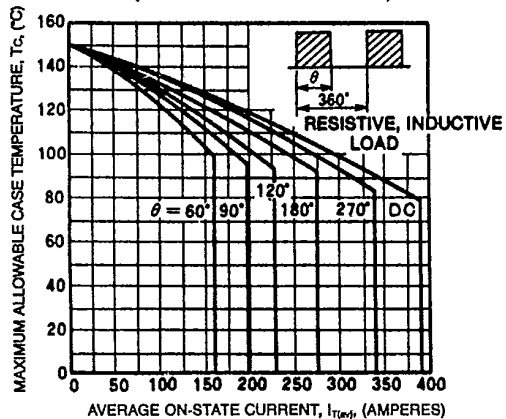
MAXIMUM ALLOWABLE CASE TEMPERATURE (RECTANGULAR WAVEFORM)
