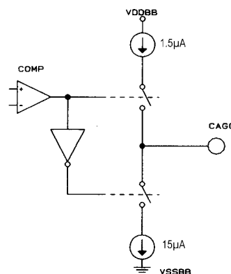
Figure 3 CAGC Pin
