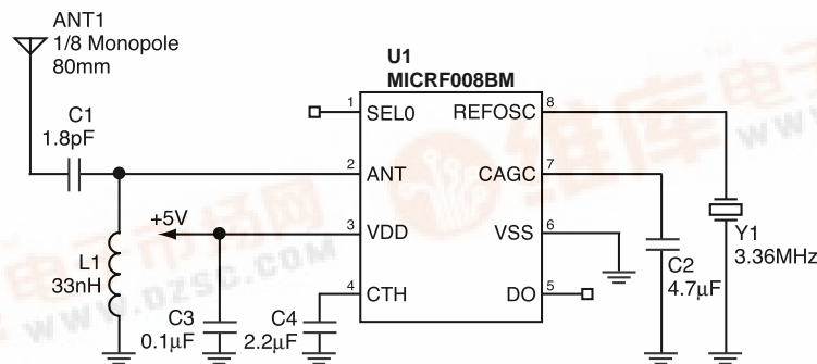
433.92MHz Receiver
