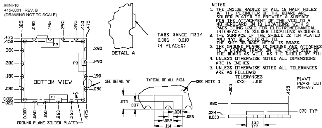
PHYSICAL DIMENSIONS
