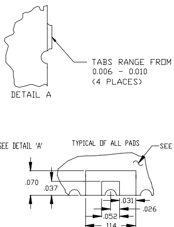
PHYSICAL DIMENSIONS
