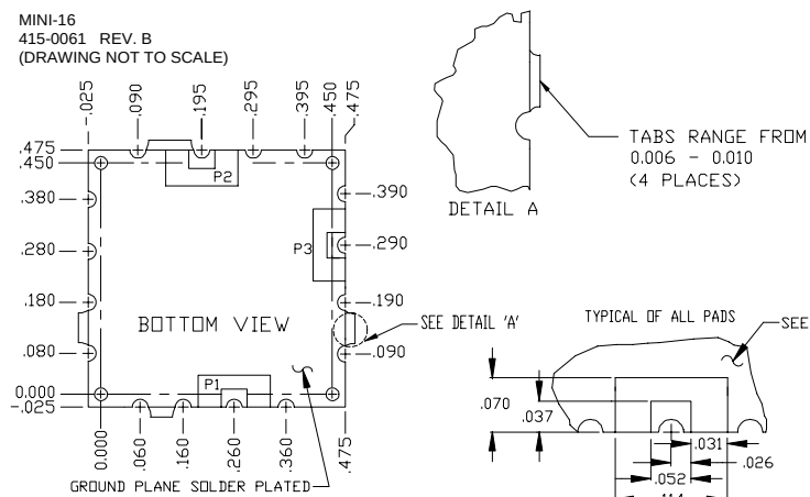
PHYSICAL DIMENSIONS
