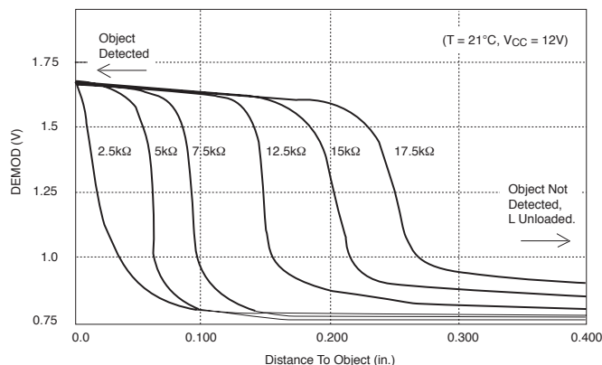
Demodulator Voltage vs. Distance for Different RF
